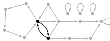
Fig. 2. Cycle C_0 .
