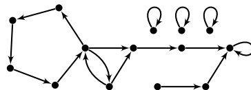
Fig. 9. Graph H_2^2 .
