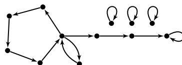
Fig. 7. Graph H_2^1 .
