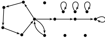
Fig. 14. Graph G_7 .
