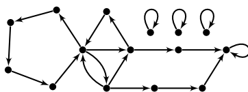
Fig. 1. Graph G = (V, E) .
