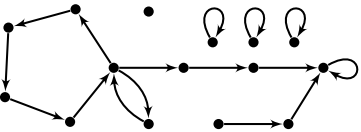
Fig. 13. Graph G_8 .
