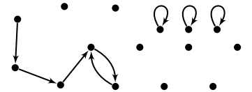
Fig. 17. Graph G_4 .
