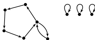
Fig. 5. Graph H_2^0 .
