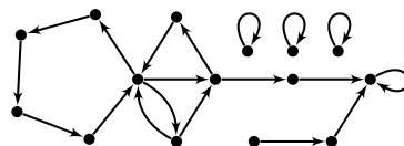
Fig. 11. Graph H_2^3 = G_9 .
