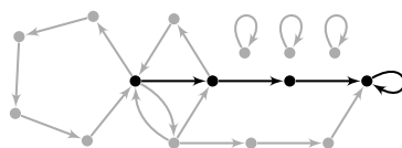
Fig. 6. Path P_1 .
