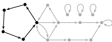
Fig. 4. Path P_0 .
