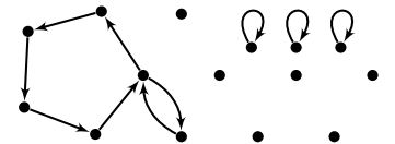
Fig. 16. Graph G_5 .
